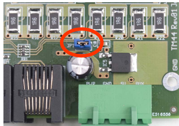
Abb. 5: Power Jumper JP1
